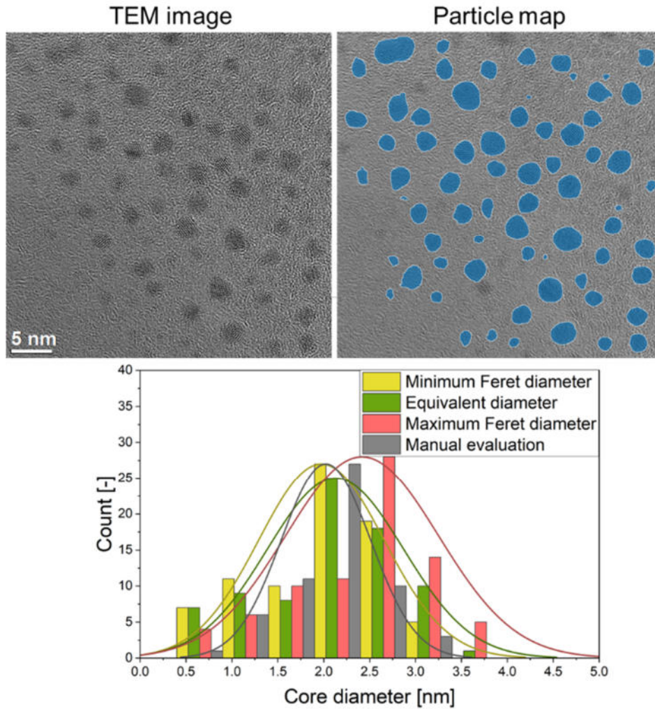
Figure 4: Particle size distribution results (minimum and maximum Feret diameters and equivalent diameter) obtained by the automated image processing routine of a TEM image of ultrasmall gold nanoparticles together with a manual determination of the distribution of the particle equivalent diameters by a human evaluator for comparison.
