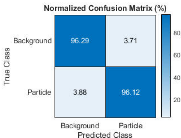
Figure 8: Normalized confusion matrix for the trained network on the test dataset, showing the percentage of pixels in a given class in the ground truth (True Class) being allocated to different classes by the network (Predicted Class).
