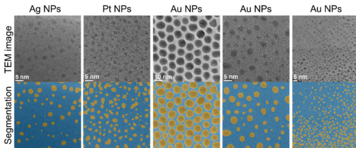
Figure 3: Representative examples of the separation of metallic nanoparticles from the background (segmentation).
