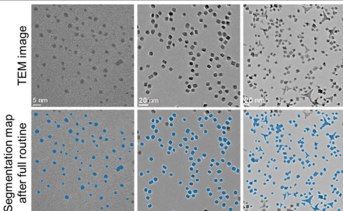
Figure 6: Analysis of TEM images with different shapes of gold (left) and platinum (centre and right) nanoparticles.
