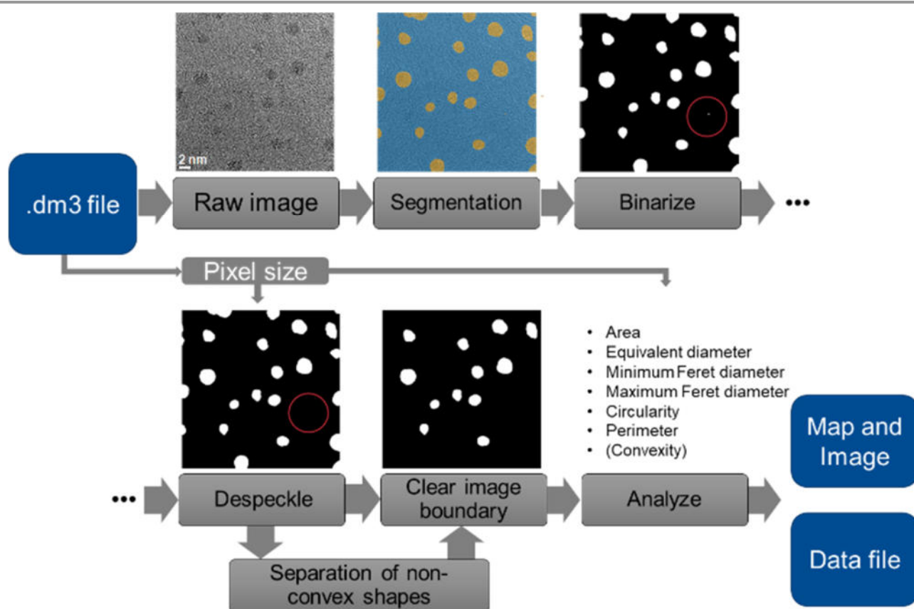
Figure 1: Illustration of the TEM image processing routine. A typical speckle that was removed is labelled by a red circle.
