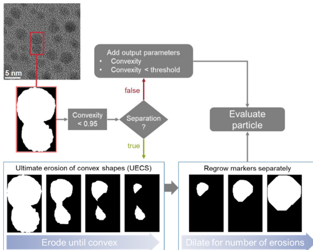
Figure 2: Illustration of the implemented options to deal with overlapping particles and illustration of the erosion and dilation process in particle separation.
