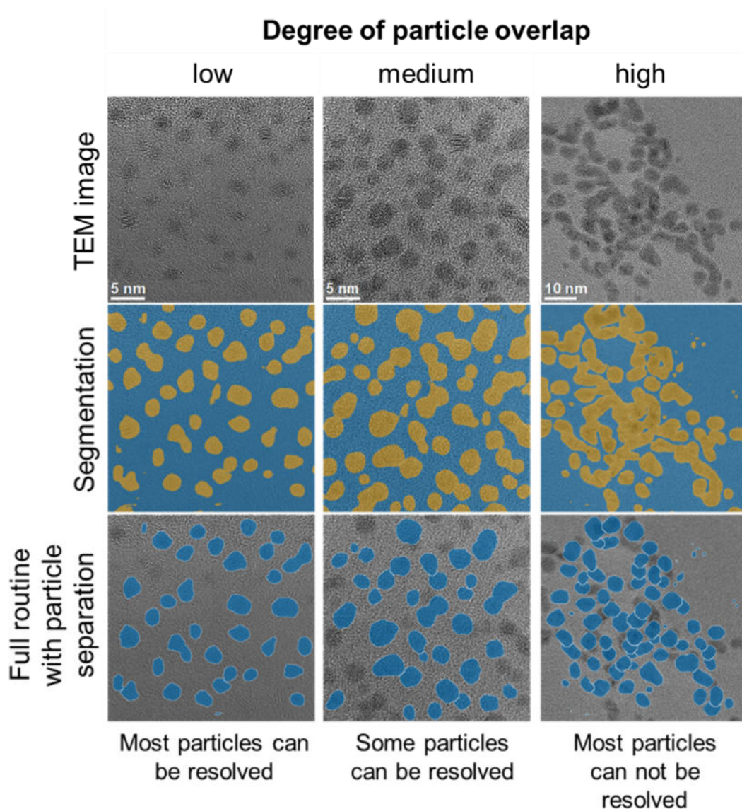
Figure 7: Examples of images of ultrasmall gold nanoparticles that can and cannot be properly evaluated due to different degrees of particle overlap. The segmentation image (middle) shows pixels in the foreground in yellow. The particle separation map (bottom) shows individually identified particles in blue.
